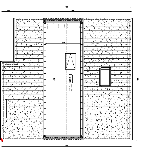
zolderplan lot 2
