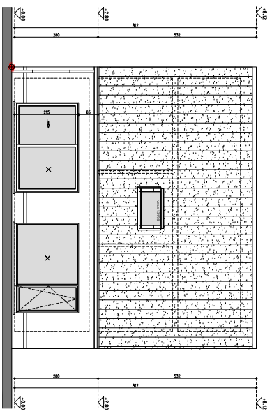
doorsnede 2-2 lot 2
