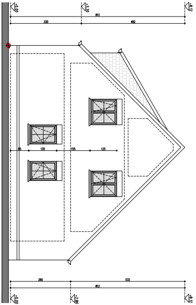
doorsnede 1-1 lot 2
