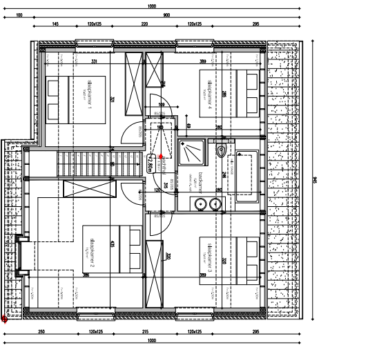
verdiepingsplan lot 2
